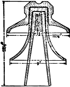
FIG. 18.—SECTION OF HIGH-TENSION INSULATOR.
